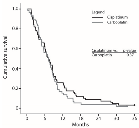
Figure S9.2 Overall survival for panel-consensus LCNEC (N=128) according to treatment by cisplatin or carboplatin doublet chemotherapy
