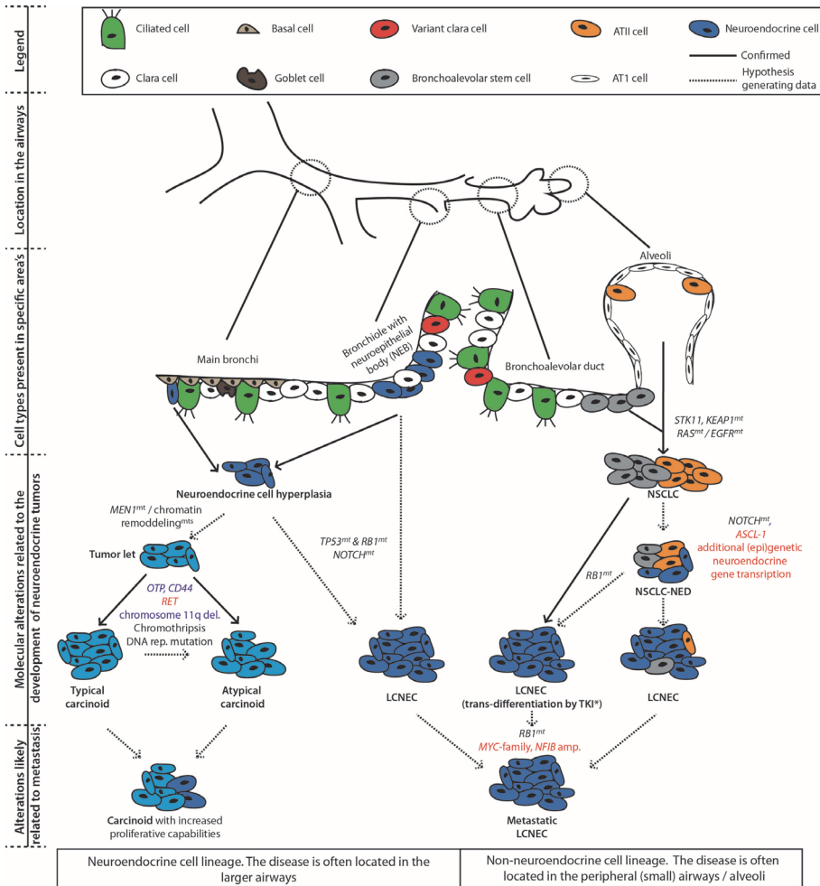
Figure 11.2 A putative overview of molecular alterations in proposed pulmonary cells of origin leading to carcinoid and LCNEC, molecular alterations related to metastatic disease are given Abbreviations: alt, alternative; morph, morphology; TKI, tyrosine kinase inhibitor; del, deletion; amp, amplification; mt, mutation; NSCLC-NED, non-small cell lung carcinoma with neuroendocrine differentiation; LCNEC, large cell neuroendocrine carcinoma; rep, replication
