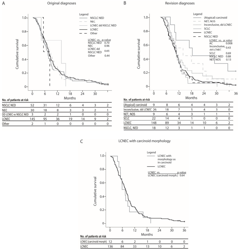
Figure S10.1 A ) OS according to the original established diagnosis in patients included in the panel consensus revision (n=232). B ) OS according to the panel consensus diagnoses, patients with carcinoids have longer OS. C ) Comparison of consensus LCNEC diagnoses versus consensus LCNEC with carcinoid morphology, no differences were observed in prognosis Abbreviations: No, number of; LCNEC, Large cell neuroendocrine carcinoma; NSCLC NED, non-small cell lung carcinoma with neuroendocrine differentiation; NEC, neuroendocrine carcinoma; dd, differential diagnosis; NET NOS, neuroendocrine tumor not otherwise specified; SCLC, small cell lung carcinoma; OS, overall survival
